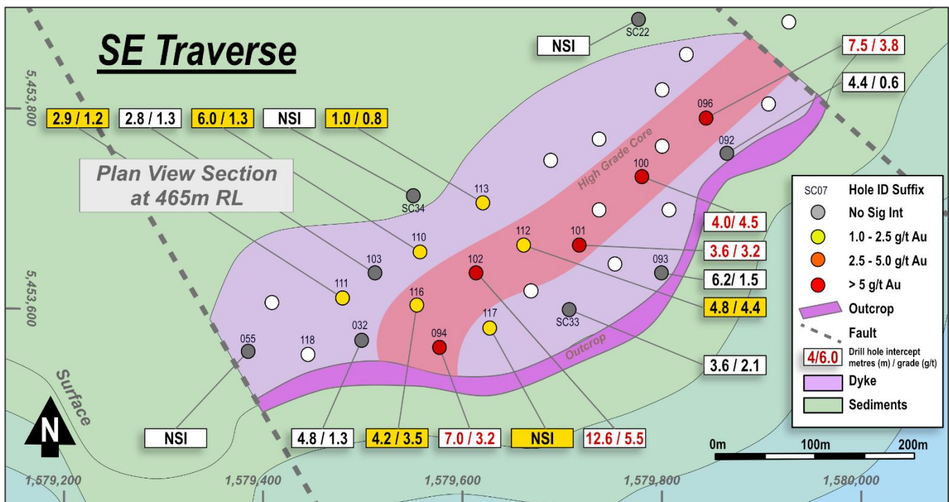
Figure 1: Plan section view of SE Traverse ore zone showing previous, current and planned drillhole intercepts.
