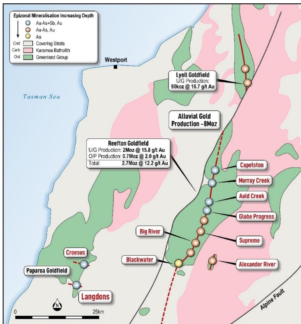
Figure 1: Simplified Geology plan of Reefton, Lyell and Paparoa goldfields.
